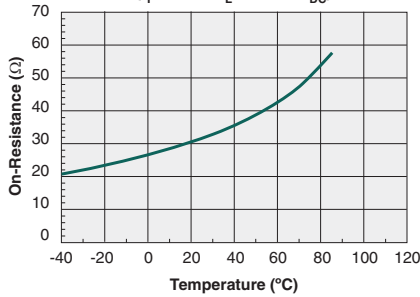
Typical On-Resistance vs. Temperature ( I_F=5mA, I_L=100mA_{DC} )
