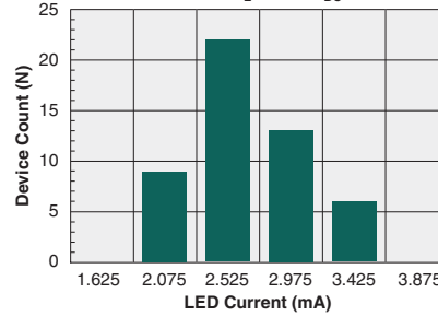
Typical I F for Switch Dropout (N=50, I L =50mA DC )
