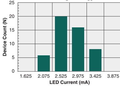
Typical I F for Switch Operation (N=50, I L =50mA DC )
