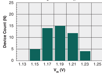
Typical V_{IN} for Switch Dropout (N=50, I_L=100mA , T_A=25^\circ C )
