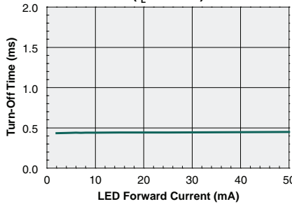
Turn-Off Time vs. LED Forward Current ( I_L=100mA )
