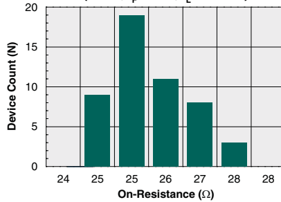
Typical On-Resistance Distribution (N=50, I F =0mA, I L =100mA)
